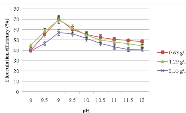
Figure 7: Flocculation tests of Scenedesmus obliquus at alkaline pH
