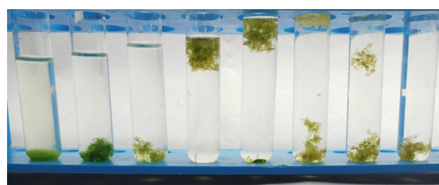
Figure 8: Flocculation efficiency of Scenedesmus obliquus at alkaline pH with 0.63 g/L initial biomass concentration
