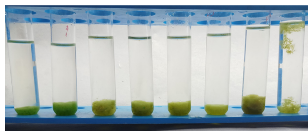
Figure 6: Flocculation efficiency of Scenedesmus obliquus at acidic pH with 0.63 g/L initial biomass concentration
